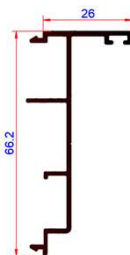
PROFILE # : AF-7304 DESCRIPTION : Sash Adapter WEIGHT : 0.435 KG/M
