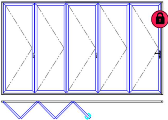
5 SASHES FOLDING DOOR
