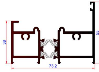
PROFILE # : AF-7303 DESCRIPTION : Bottom Frame WEIGHT : 1.763 KG/M
