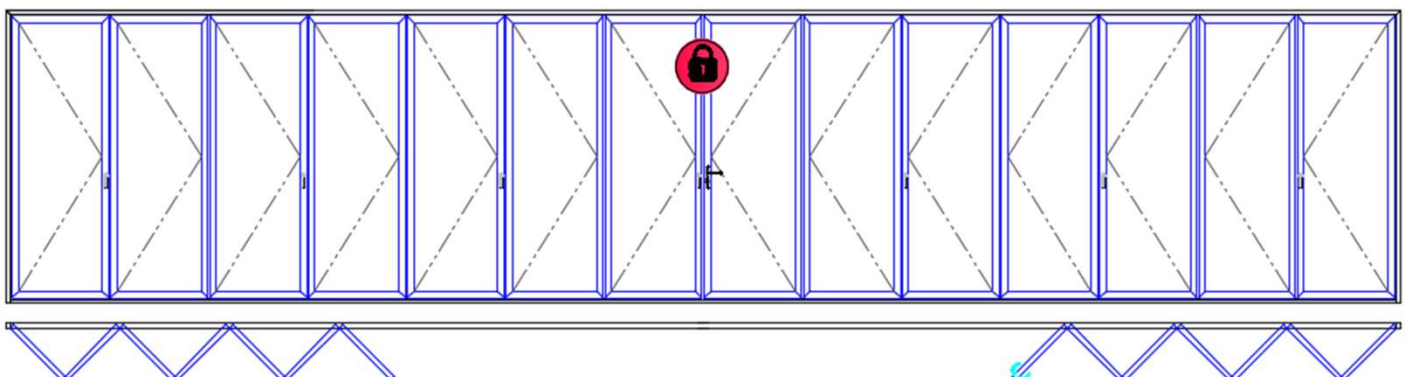
7+7 SASHES FOLDING DOOR
