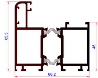
PROFILE # : AF-7306 DESCRIPTION : Vertical Sash Profile WEIGHT : 2.057 KG/M
