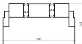
AF-CT1882F3 Smart Attached Three Upper Rail Weight : 5.77 kg/m
